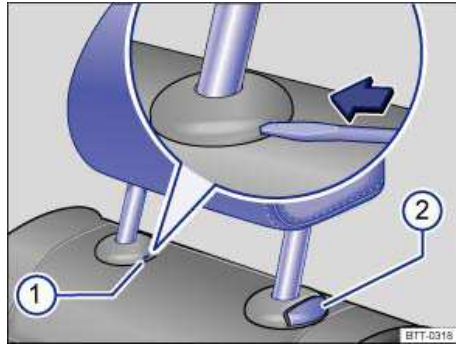
Fig. 66 Removing the rear head restraints.
