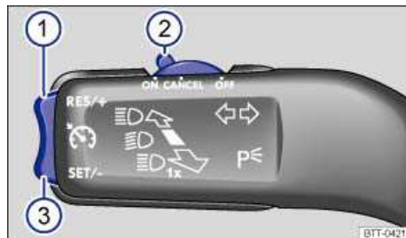
Fig. 168 On the left side of the steering column: Cruise control buttons and switches.
