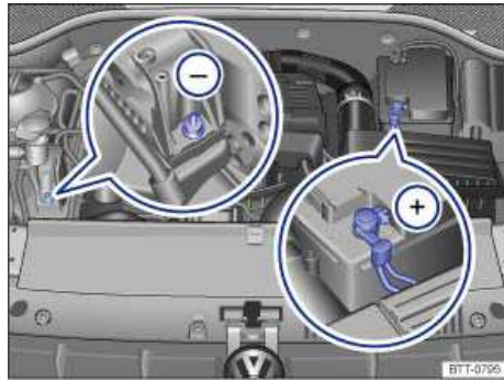
Fig. 218 In the engine compartment (1.8 liter engine): Positive jump-start terminal + and negative jump-start terminal -.
