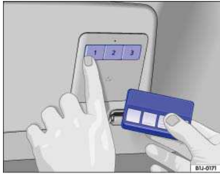
Fig. 55 To program: Simultaneously press the buttons for the HomeLink Universal Transmitter and the remote control.
