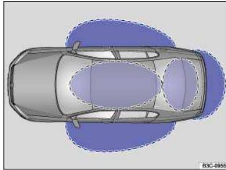
Fig. 40 Ranges of the Keyless Access with push button start. Outside the vehicle: Unlocking range. Inside the vehicle: Starting range.
