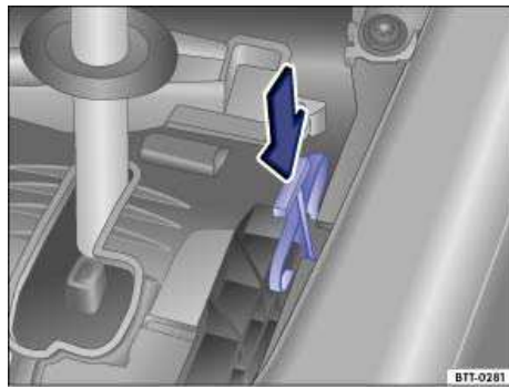
Fig. 204 Releasing the selector lever lock.
