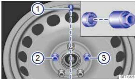
Fig. 210 Changing a wheel: tire valve 1 and installation points for the anti-theft wheel bolt 2 or 3 (where applicable).
