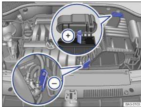
Fig. 220 In the engine compartment (3.6 liter engine): Positive jump-start terminal + and negative jump-start terminal -.
