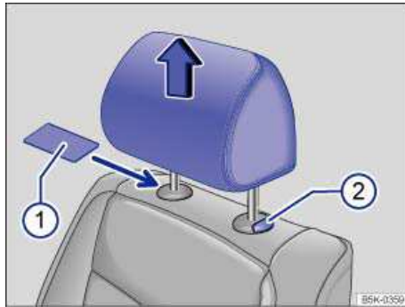
Fig. 65 Removing the front head restraints.
