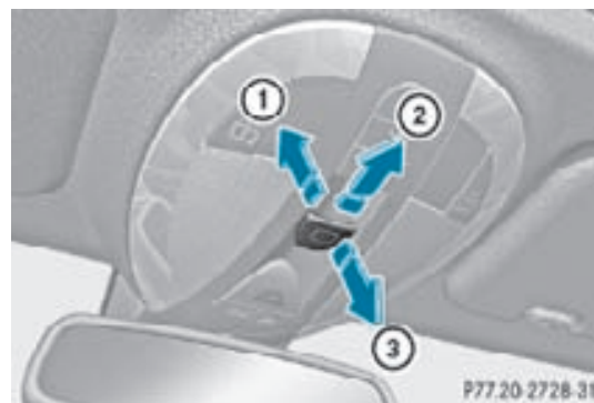
Sunroof switch
