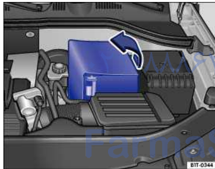
Fig. 146 In the engine compartment: Open the sleeve covering of the vehicle battery.
