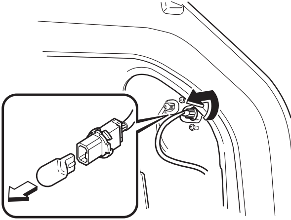
Brake lights/Taillights/Rear side-marker lights (Bulb type)
